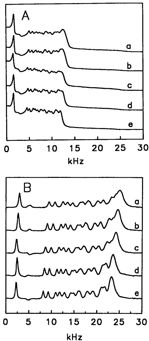
FIGURE 9 (A) Right-hand side of ^2\text{H} -NMR powder spectra of DPPC- \text{d}_{62} at 50^\circ\text{C} as a function of TA concentration. (a) DPPC; (b) 120/1 DPPC/TA; (c) 60/1 DPPC/TA; (d) 30/1 DPPC/TA; (e) 15/1 DPPC/TA. (B) dePaked spectra of the data shown in A.
