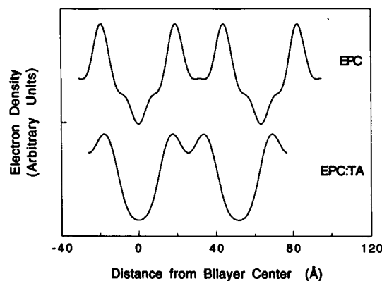
FIGURE 14 Electron density profiles for EPC in water ( top profile ) and EPC in 0.1 mM mM TA ( bottom profile ).
