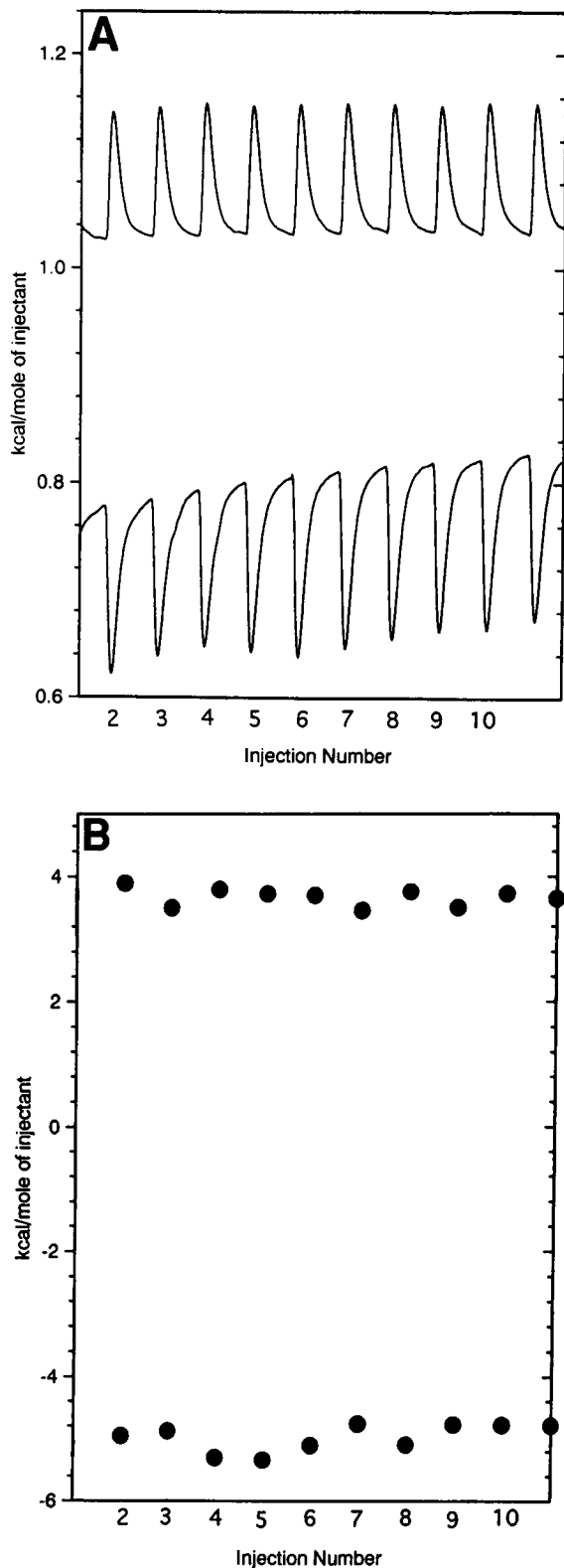
FIGURE 8 (A) Heats of solution and binding of tannic acid to EPC large unilamellar vesicles. Injections of 0.2 \mu\text{L} of 25 mM tannic acid in 1 mM NaCl, 5 mM HEPES, pH 7.0 into 1 mM NaCl, 5 mM HEPES, adjusted to pH 7.0 yield endothermic transitions ( top trace ). Injections of 0.2 \mu\text{L} of 25 mM tannic acid (in 1 mM NaCl, 5 mM HEPES, pH 7.0) into 6.6 mM EPC in 1 mM NaCl, 5 mM HEPES, pH 7.0 yield exothermic transitions ( bottom trace ). (B) Heats of solution ( top ) and binding ( bottom ) of TA calculated from the data presented in A.
